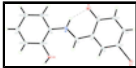
Fig. 1. The molecular structure of the title compound, with 50% probability displacement ellipsoids and the atom-numbering scheme. Hydrogen bond is shown as dashed lines.
